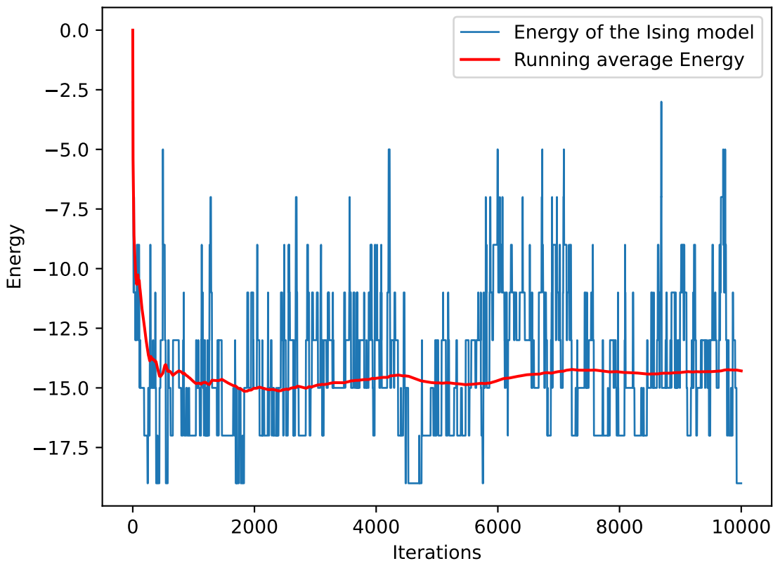
Evolution of a stochastic simulation of the 1D Ising model, at \beta = 1 J = 1 h = 0
